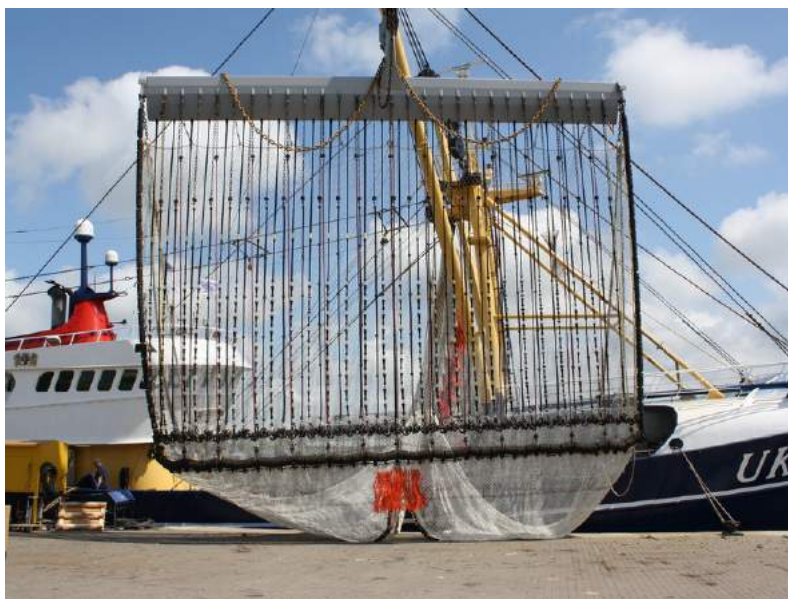
Figure 3. Pulse trawl fishing gear: The electrodes generate an electric pulse to catch flatfish.
